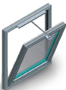
BOTTOM HUNG OPENING INWARD
